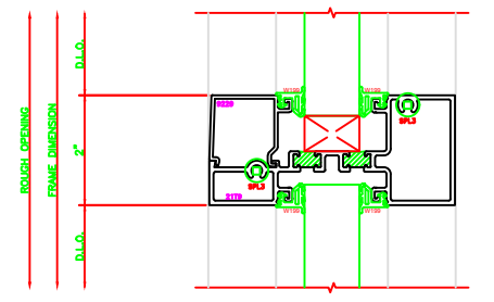
501 O.G. HORIZONTAL SERIES: 403X - 2" X 4 1/2" SCREWSPLINE
