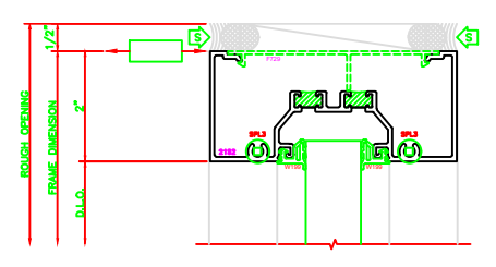
101 O.G. HEAD SERIES: 403X - 2" X 4 1/2" SCREWSPLINE
