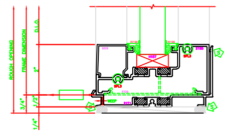
201 O.G. SILL SERIES: 403X - 2" X 4 1/2" SCREWSPLINE
